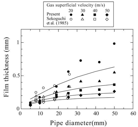
Fig. 13. Effect of pipe diameter of average film thickness and comparison with predictions of correlations of Asali et al. (1985) and Kosky (1971).
