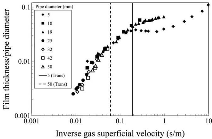
Fig. 12. Relationship between dimensionless film thickness and inverse gas superficial velocity – liquid superficial velocity = 0.1 m/s.
