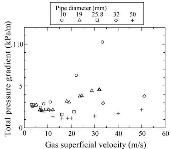
Fig. 14. Total pressure gradient versus gas superficial velocity (liquid superficial velocity = 0.1 m/s).
