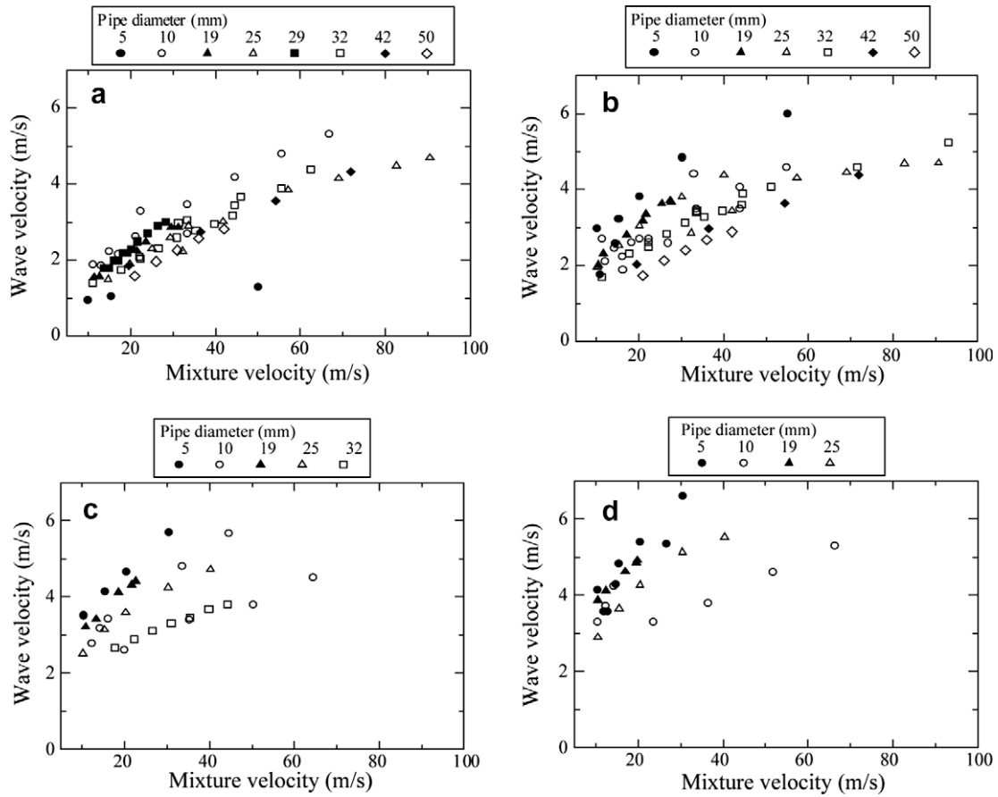
Fig. 18. Effect of pipe diameter on velocity of disturbance waves at different liquid flow rates. ((a–d) corresponds to liquid superficial velocities of 0.03, 0.1, 0.2 and 0.4 m/s, respectively).
